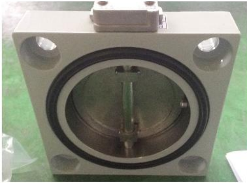
6" GE Square BFV & rectangle shape BFV.
