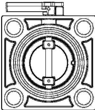
Bolting circle PCD 160
